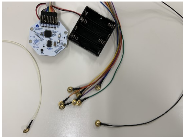
Figure 5. The OpenBCI Cyton board.
